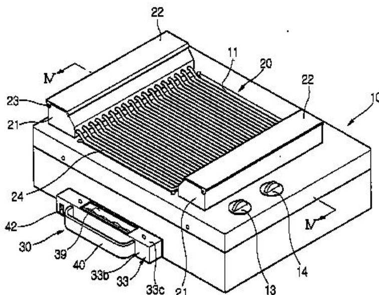
Example of an open grill (from EP1417918 by Samsung Electronics Co., Ltd.)
