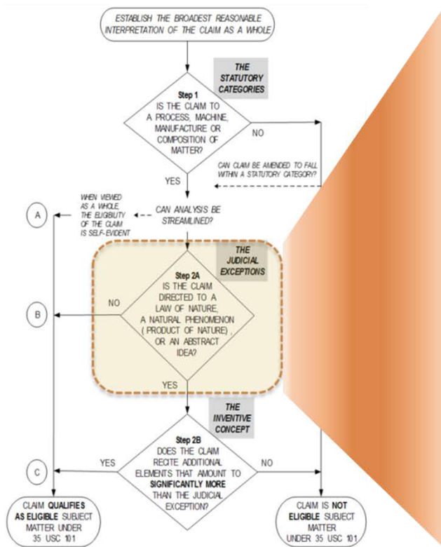
MPEP flowchart
